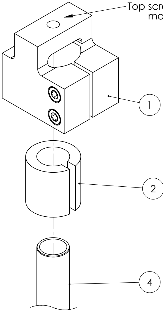
Bicycle Fork Steer Tube
