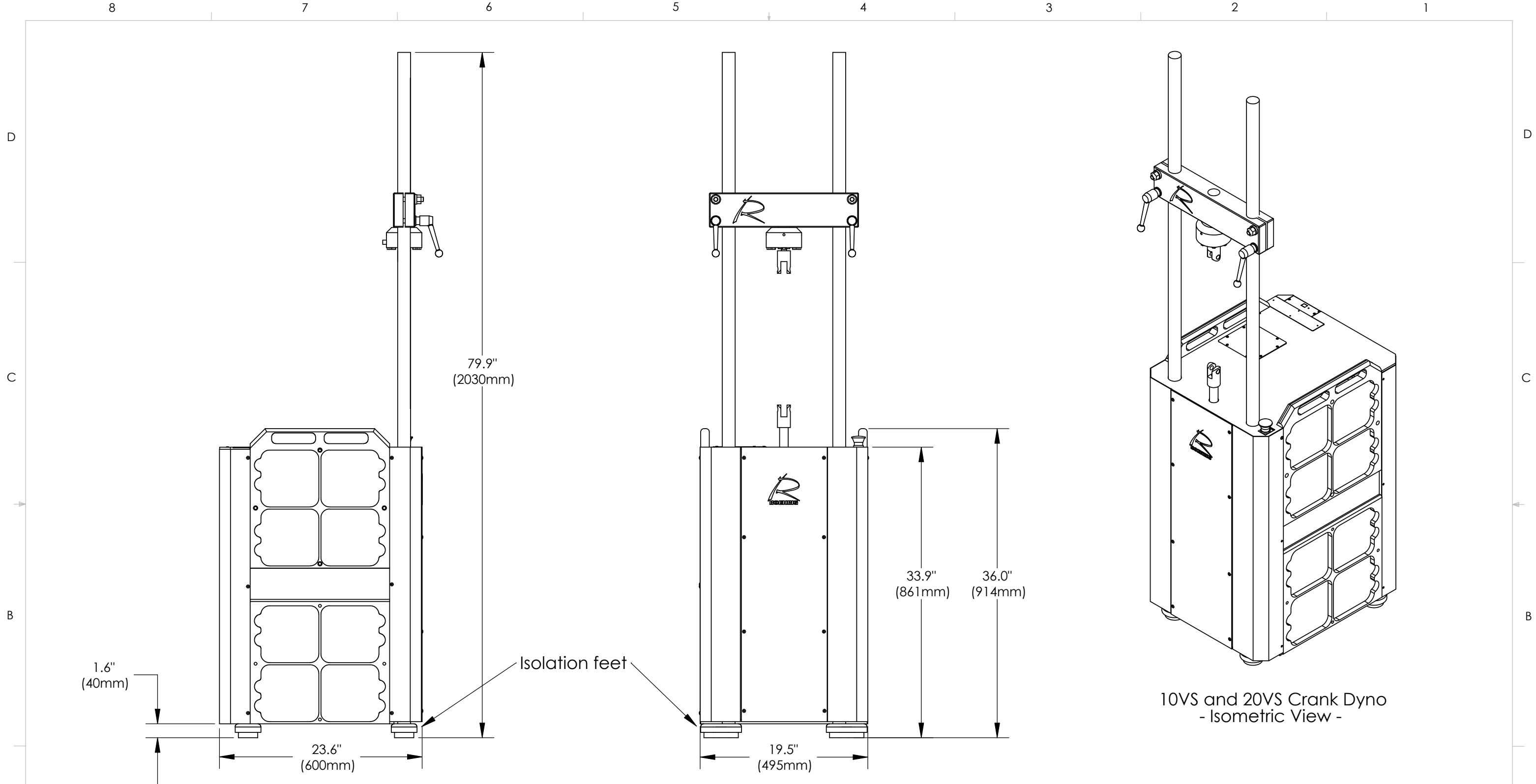
10VS and 20VS Crank Dyno - Side View -
