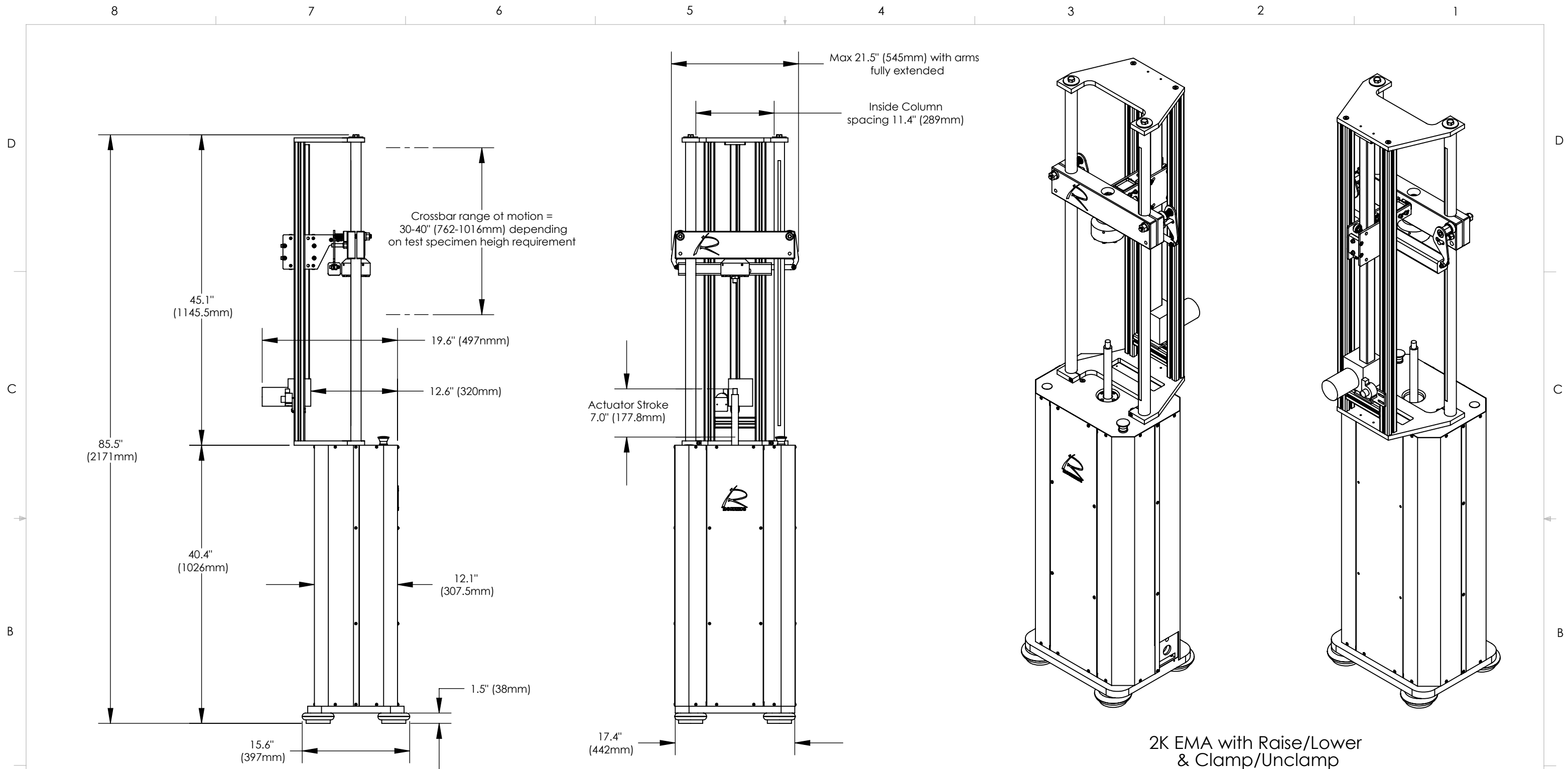
2K EMA with Raise/Lower & Clamp/Unclamp - Side View-
