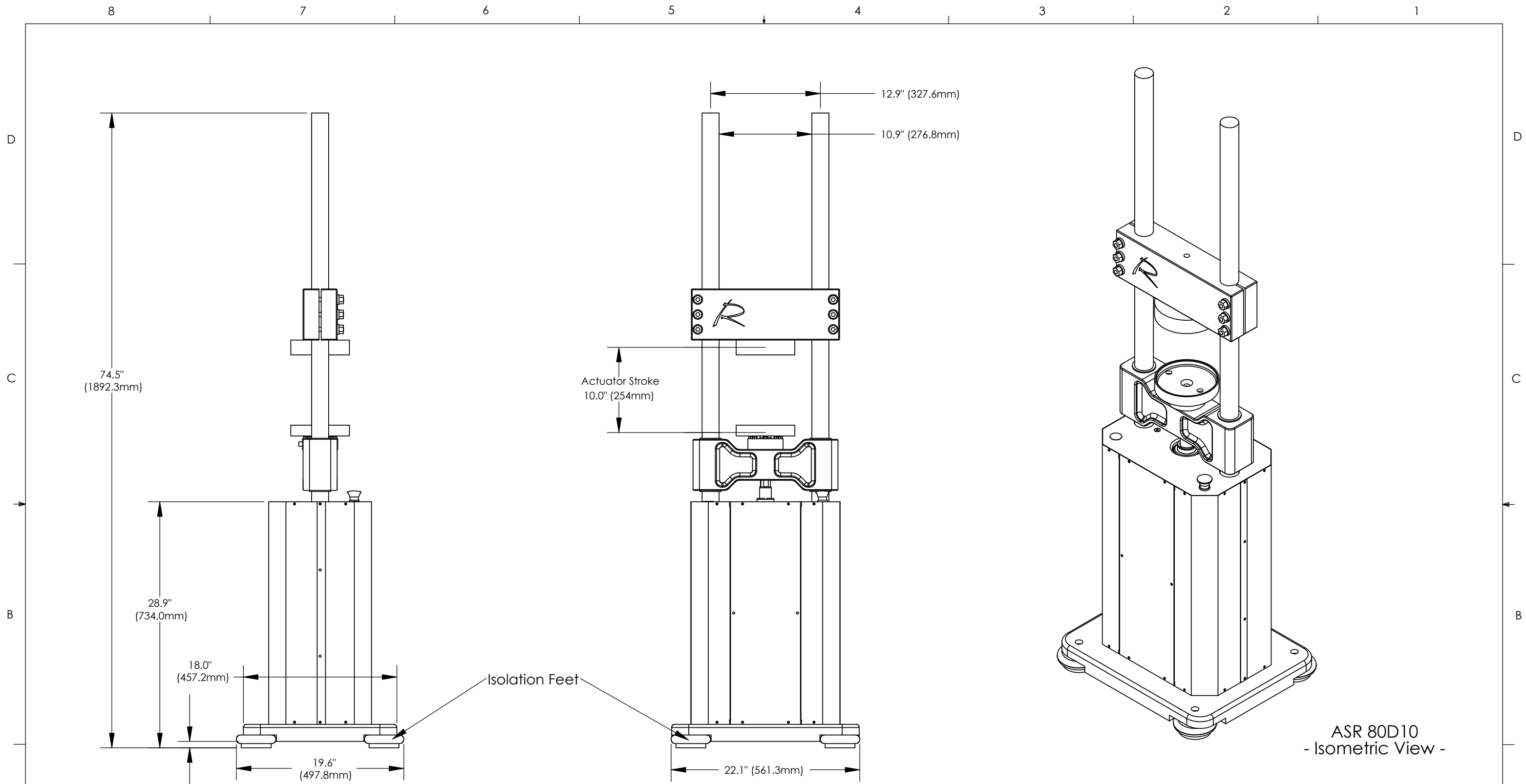
ASR 80D10 - Side View -
