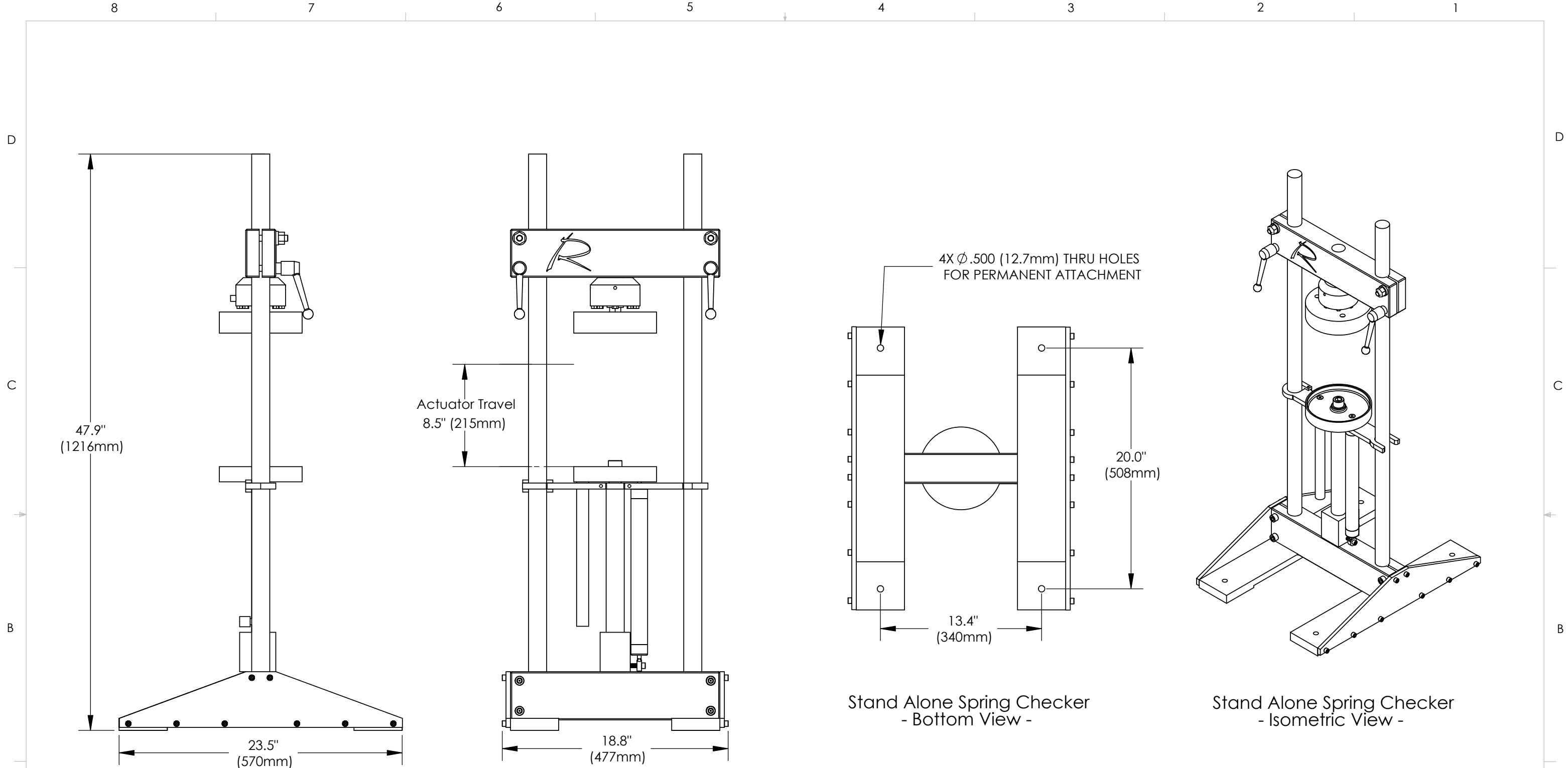
Stand Alone Spring Checker - Side View -
