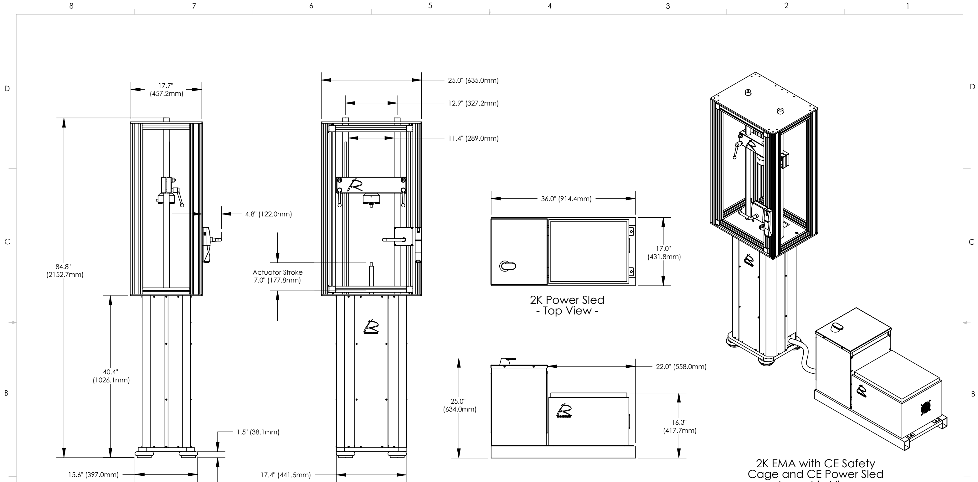
2K Power Sled - Front View -
