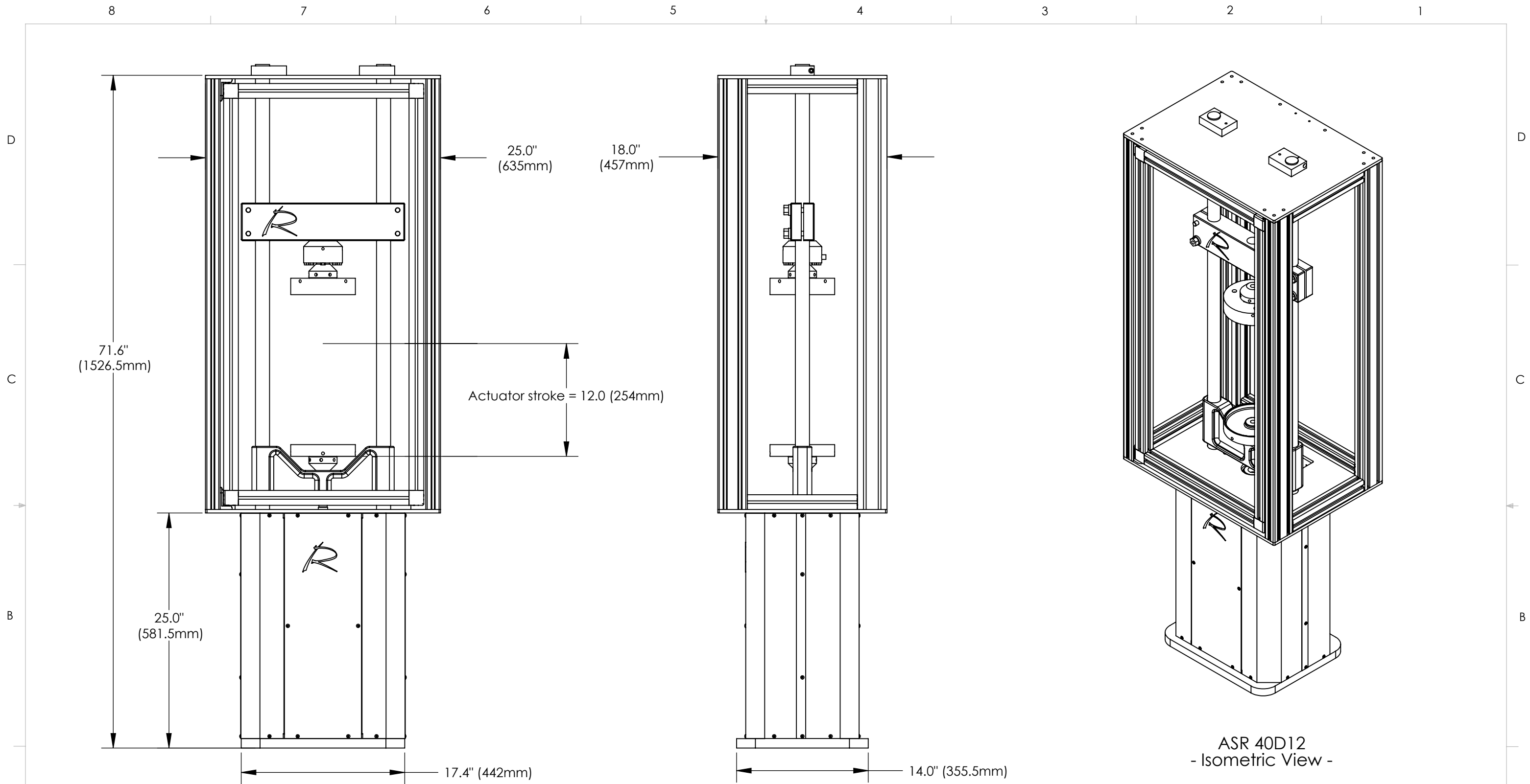
ASR 40D12 - Side View -
